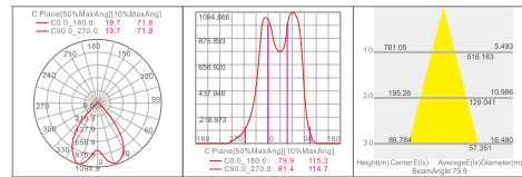
20W 80° Double Asymmetric
