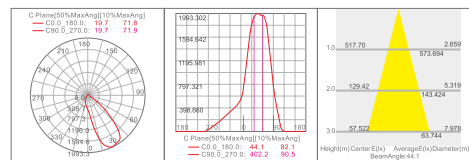
20W 50° Single Asymmetric
